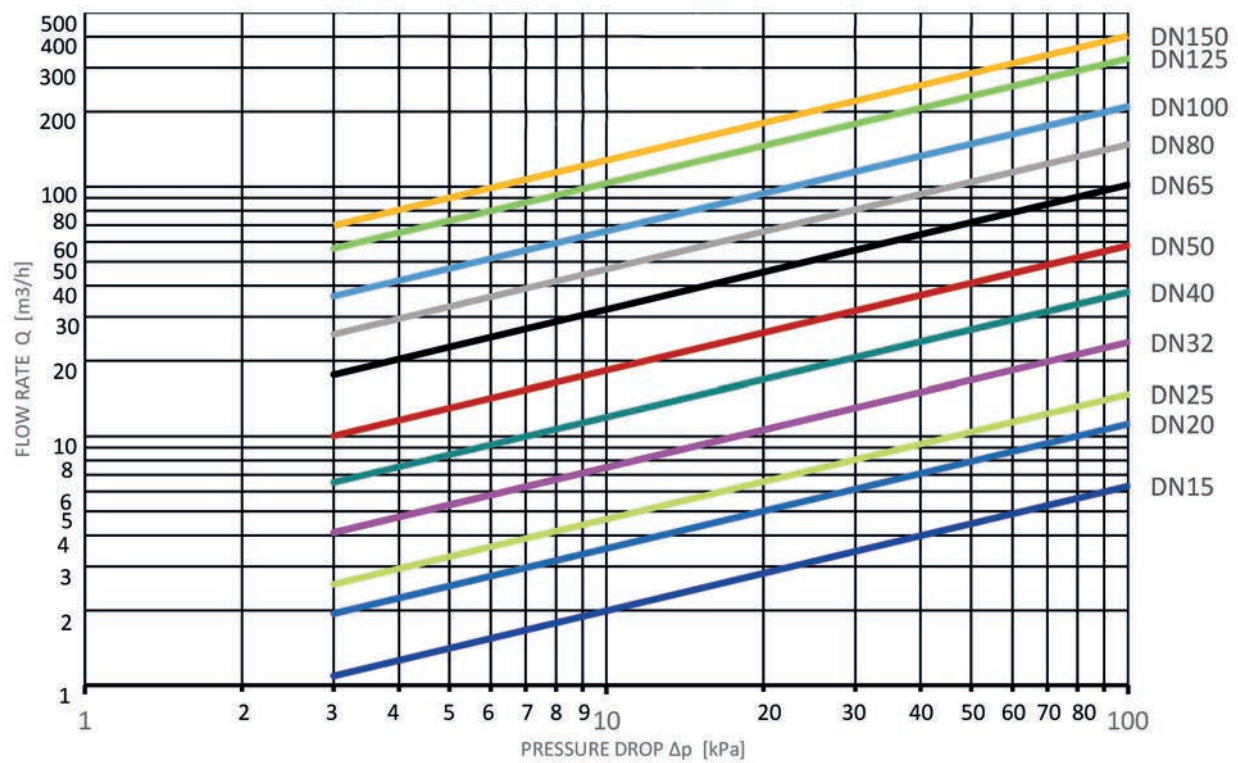
Pressure Drop Chart
